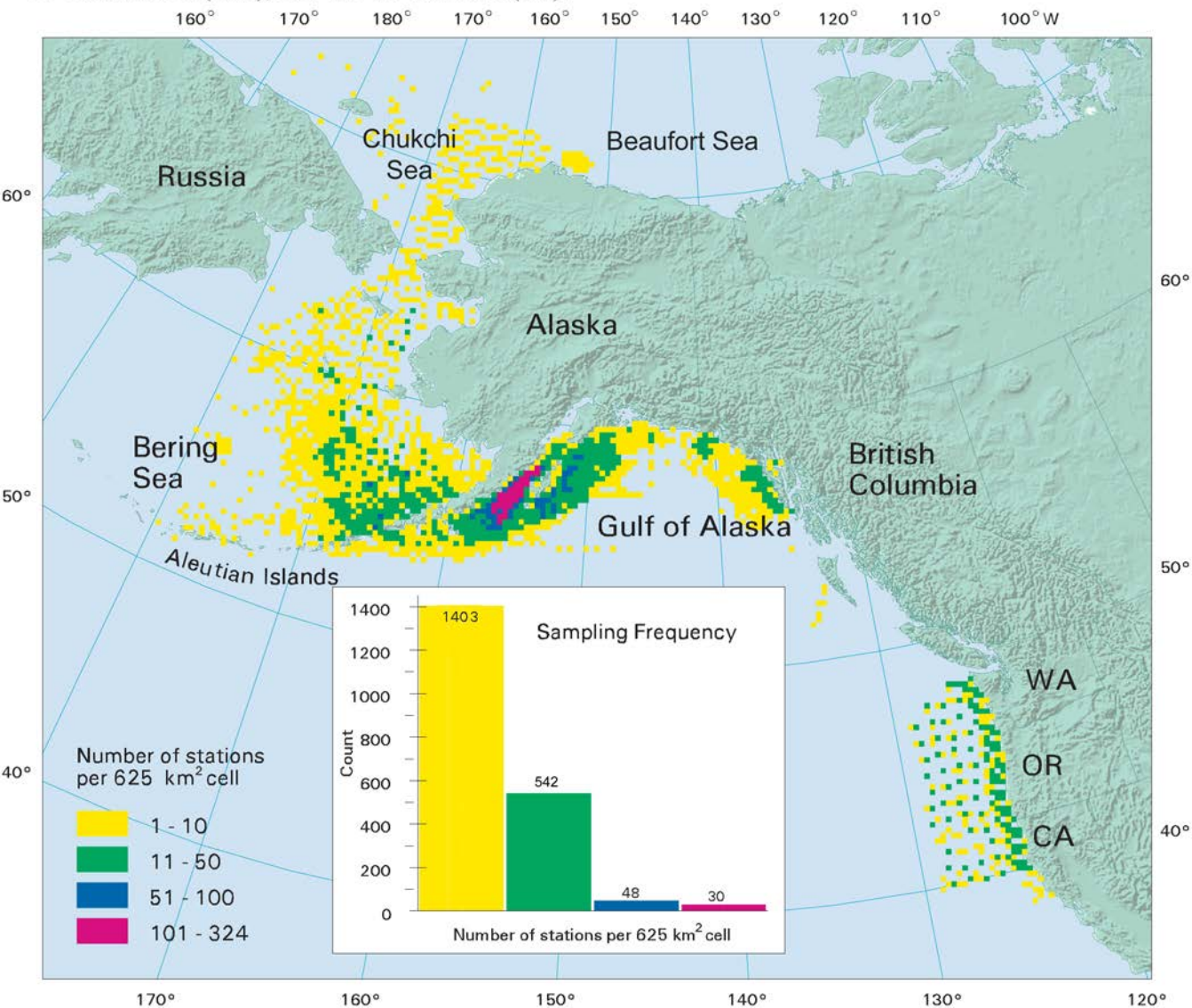
Map 9. Geographic distribution and frequency of sampling during Recruitment Processes Program ichthyoplankton surveys for 1972-2010. Area sampled is divided into 625 km 2 cells. Numbers on or over bars in histogram equal number of cells that contain 1-10 stations (yellow), 11-50 stations (green), 51-100 stations (blue), and 101-324 stations (red).
